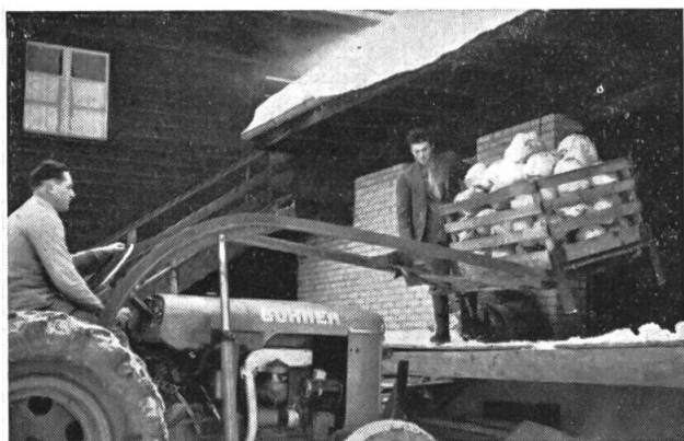
Frontlader Vogel
