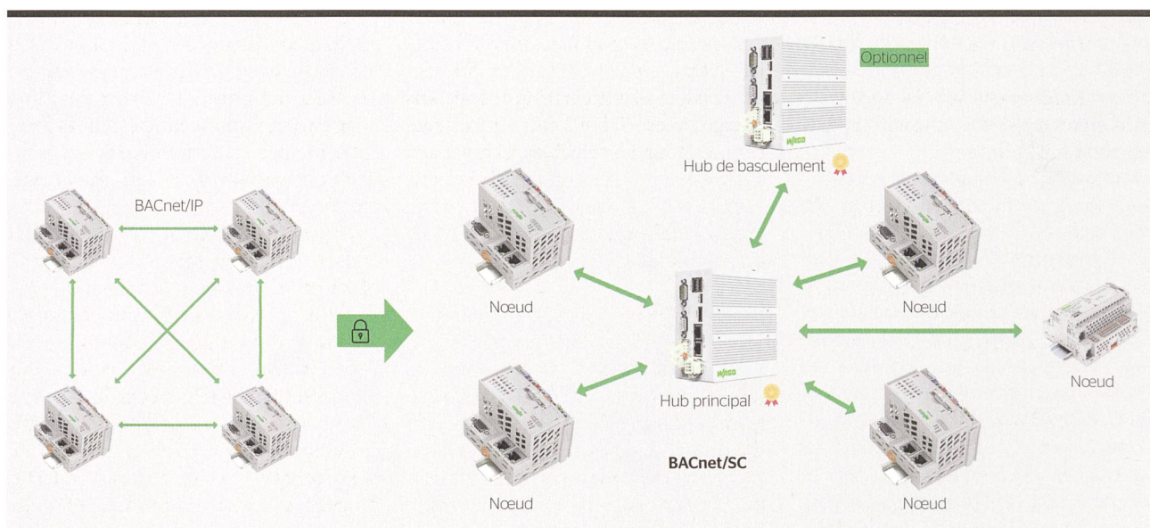
Figure 2 Comparaison des architectures BACnet/IP et BACnet/SC.
