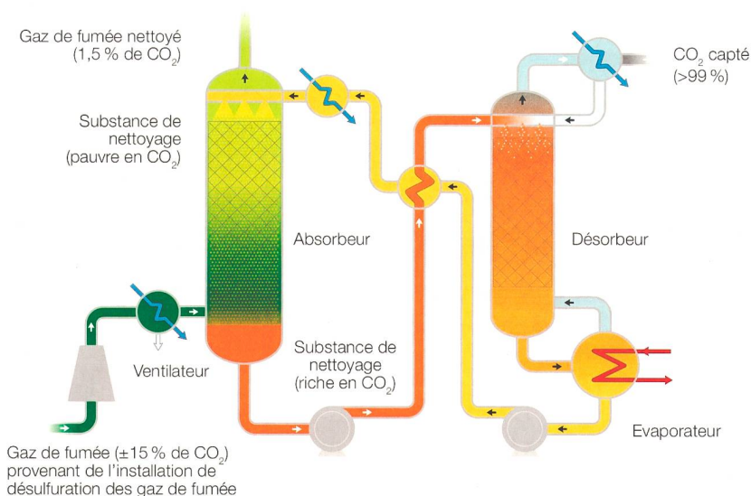
Installation pilote PCC (Post-Combustion Capture)
