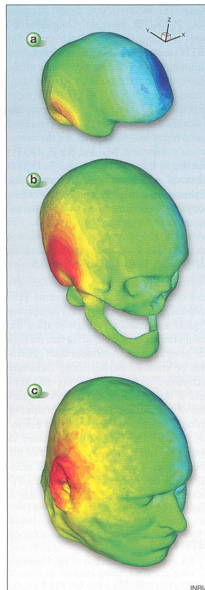
Figure 5 Normalized SAR (mesh M1, \mathbb{P}_1 -DGTD method)
