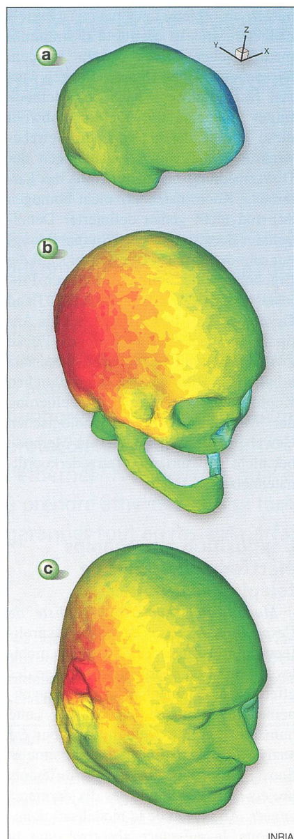
Figure 3 Normalized SAR (mesh M1, \mathbb{P}_0 -DGTD method)
