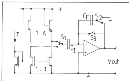
Fig. 11 Switched capacitor approach of a V_{PTAT} source [8]
