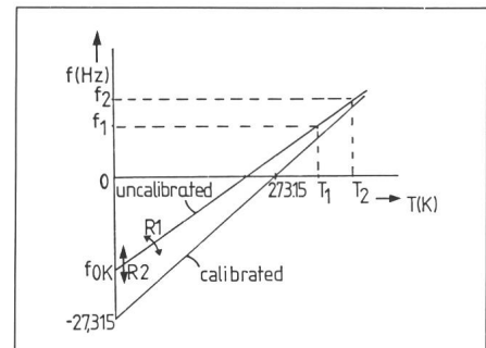
Fig. 15 Calibration of the temperature controlled oscillator
