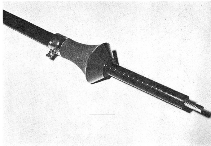
Fig. 15 Stress-Cone 20 kV
