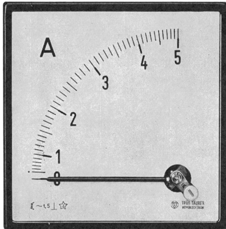
Quadrant-Instrument MINIRAMA ®
