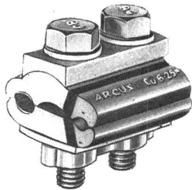
Al-Cu-Klemme
