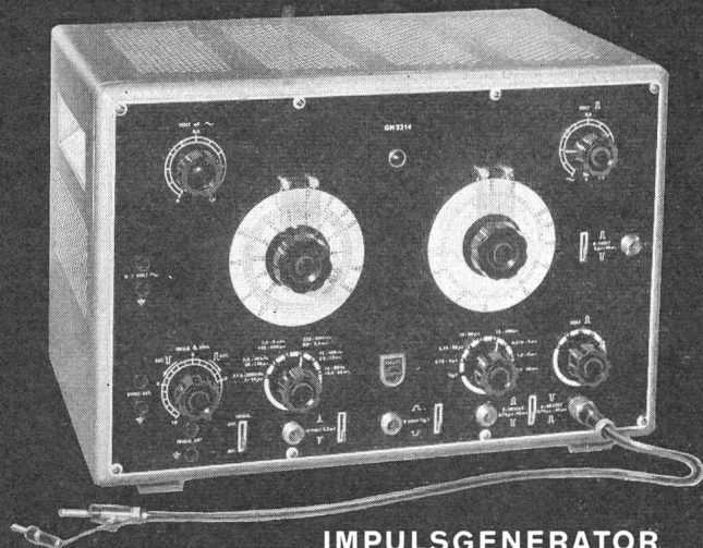
IMPULSGENERATOR GM 2314
