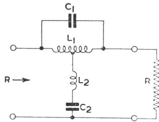
Fig. 3 Simple Phase Corrector
