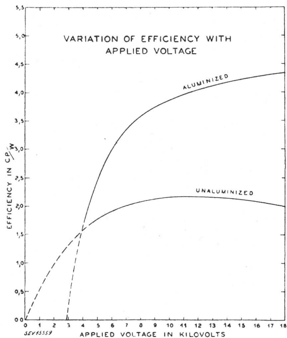
Fig. 19 Conversion Efficiency of 12-inch Kinescopes with an without Metal Film as Function of Operating Voltage
