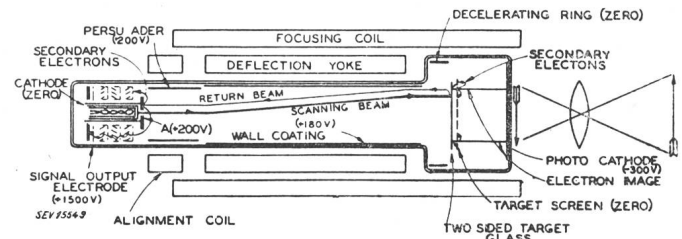
Fig. 9 The Image Orthicon (Schematic Diagram)
