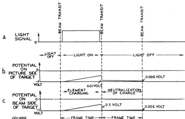
Fig. 13 Potential Variation
