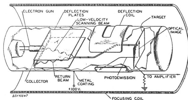
Fig. 7 Schematic Diagram of the Orthicon
