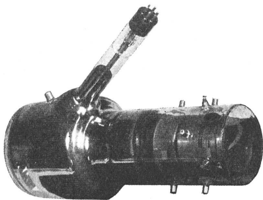
Fig. 6 An Image Iconoscope
