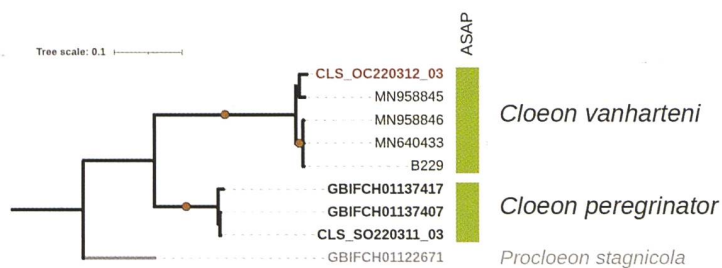
Figure 6. Bayesian majority-rule consensus COI tree including Cloeon vanharteni and C. peregrinator . Tips labelled with MN codes indicate sequences retrieved from GenBank, other codes represent newly obtained sequences from our samples. Bolded labels indicate sequences derived from Moroccan specimens, with the C. vanharteni Moroccan specimen highlighted in red. The B229 code represents a sequence originating from a specimen collected in Israel. Colored vertical boxes indicate species delimitation according to the ASAP method, with the corresponding species name next to each box. Circles on branches indicate Bayesian posterior probabilities > 0.95. The outgroup branch ( Procloeon stagnicola ) is presented in grey, along with its corresponding tip label and species name.
