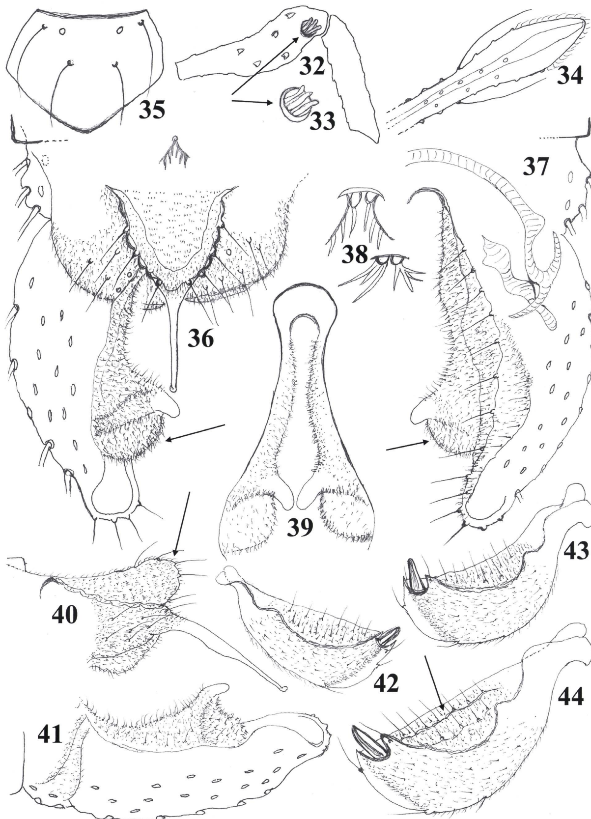
Figures 32–44. Male adult of Chaetocladius lodscrozetae sp. n.: 32–33, palpomeres 3–4 with sensilla clavata on palpomere 3; 34, last flagellomere; 35, clypeus; 36–37, hypopygium, dorsal (36) and ventral (37) with anal point and tergite IX removed; 38, virga, two aspects; 39, ventral view of inferior volsella; 40, anal point and tergite IX in lateral view; 41, left gonocoxite in lateral view; 42–44, gonostylus, lateral (42), dorsal (43) and dorso-lateral (44).
