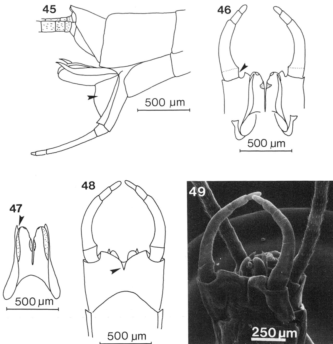
Figs. 45–49. Metrelenus balcanicus . 45: terminal abdominal segments, lateral view. 46: male genital apparatus, dorsal view. 47: penis, ventral view. 48: male genital apparatus, ventral view. 49: male genital apparatus, apico-ventral view.
