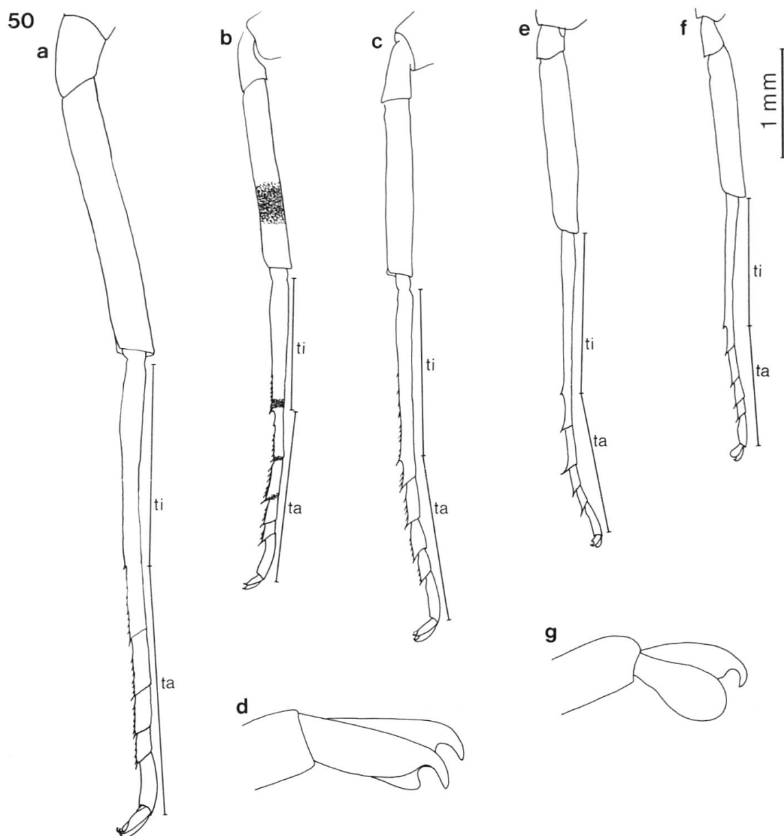
Fig. 50. Mid and hind legs of Siphonuridae males and females. a: S. aestivalis . b: S. alternatus . c: P. chelifer . d: claws of Siphonurus and Parametetus species. e: A. inopinatus . f: M. balcanicus . g: claws of Ameletus and Metreletus species.
