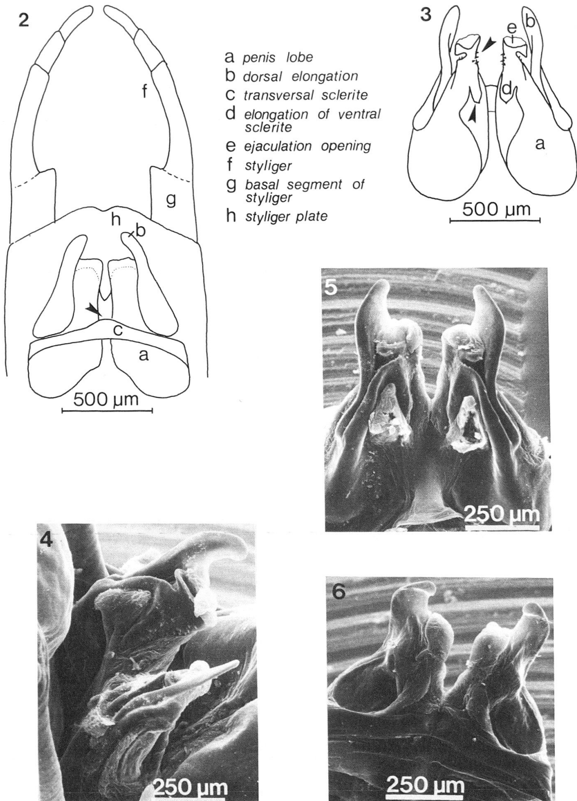
Figs. 2–6. Siphonurus aestivalis . 2: male genital apparatus (penis with styliger plate and styliger), dorsal view. 3: penis, ventral view. 4: penis, latero-apical view. 5: penis, ventral view. 6: penis, apico-dorsal view.
