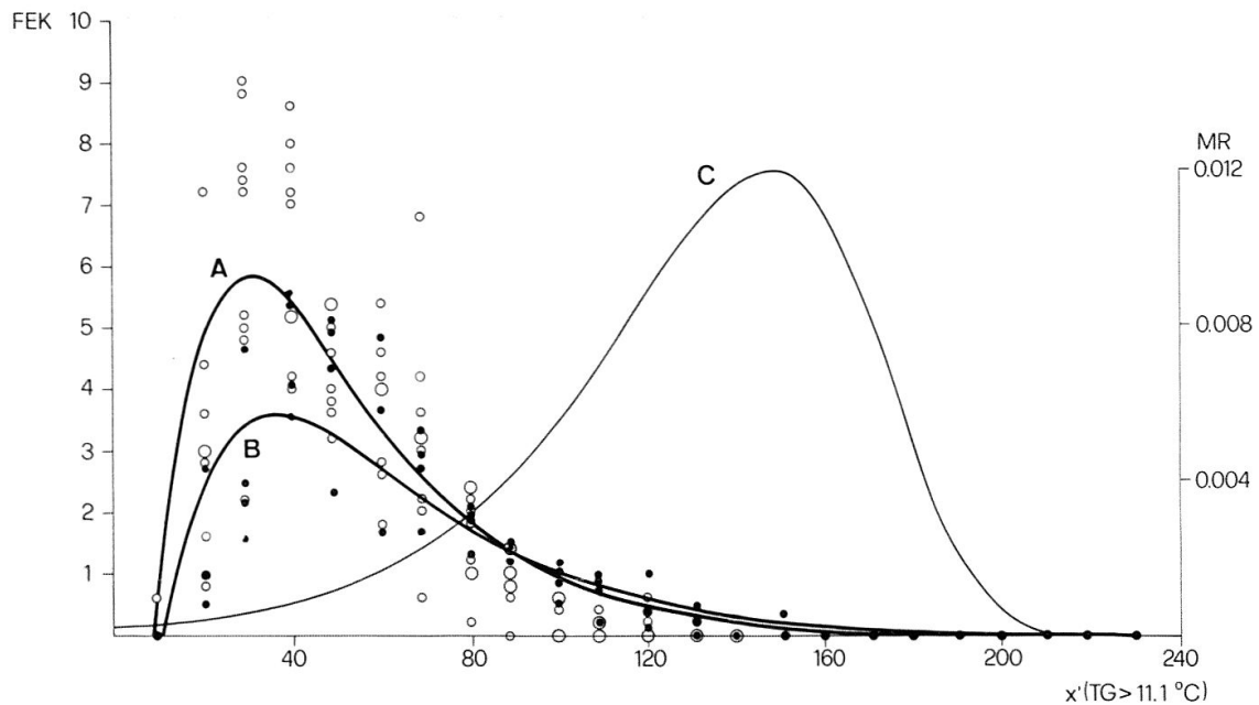
Fig. 1: Adoxophyes orana : Age (x') specific fecundity (FEK) and mortality rates (MR) for several groups of insects, kept either in an insectary (○, A) or at 25 °C (●, B). Each dot represents a calculated value for a 10 day degree period. (A : 0 \leq \text{FEK} = (0.7558 \cdot (x' - 10.54)) / (1.0488^{(x' - 10.54)}) ; B : 0 \leq \text{FEK} = (0.3752 \cdot (x' - 11.48)) / (1.0375^{(x' - 11.48)}) ; C : \text{MR} = 1 - d \cdot (\text{SURV}) / dx' = 0.00024 \cdot \text{EXP}(-0.0073 \cdot \text{EXP}(0.0335 \cdot x')) \cdot \text{EXP}(0.0335 \cdot x') ; x = age in day degrees above a 11.1 °C threshold; x' = x - 5).
