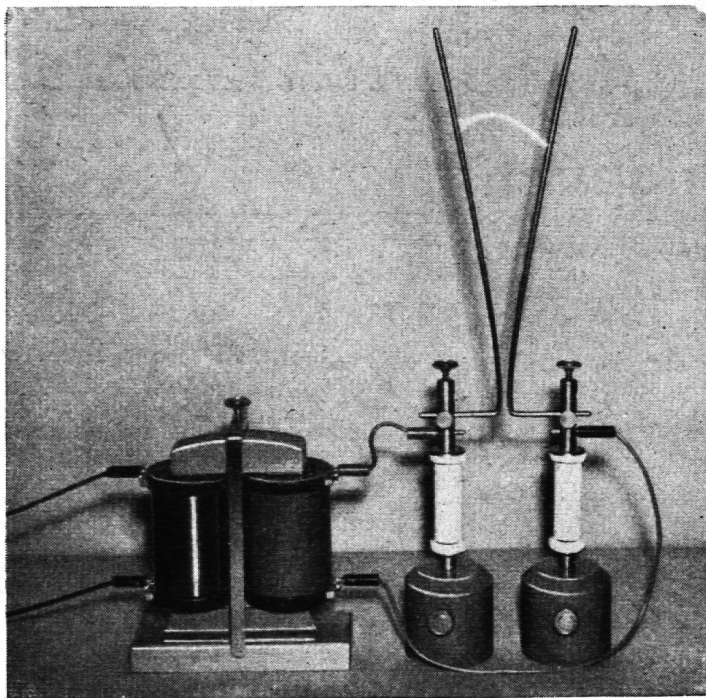
Demonstrationstransformator
