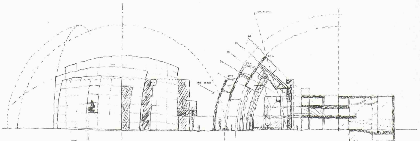
The church of the year 2000 Rome South elevation & longitudinal section 10 March 1996
