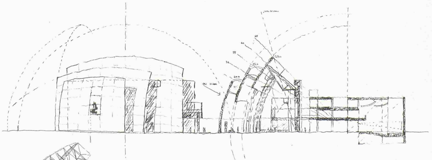
The church of the year 2000 Rome South elevation & longitudinal section 10 March 1996
