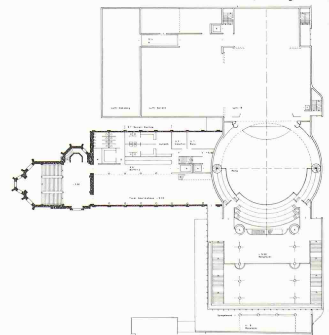
Ranggeschoss
