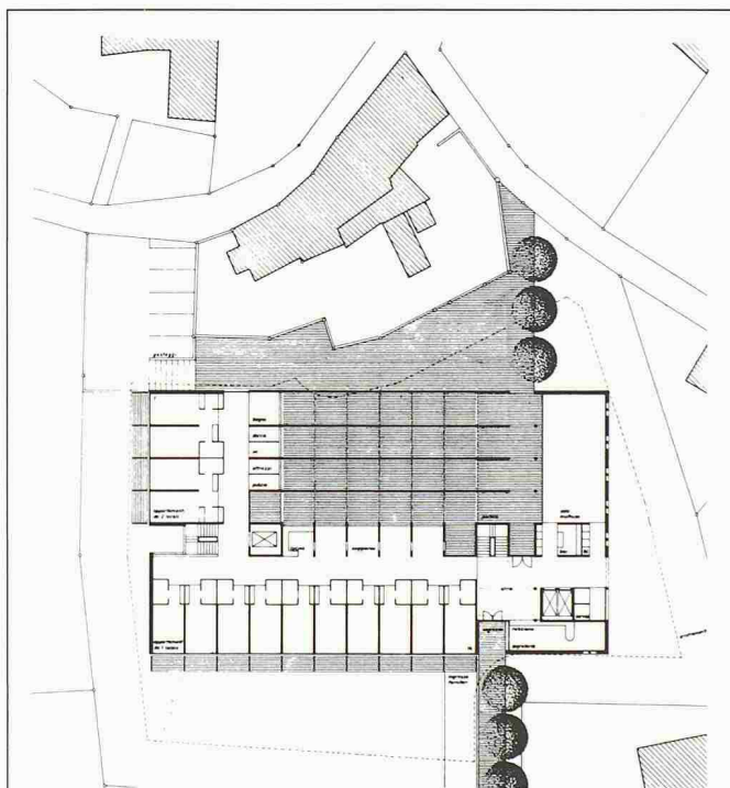
Piano terreno 1:880
