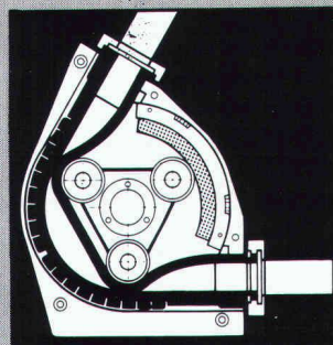
DELASCO-Pumpe
