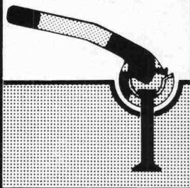
Kugelfuss- Transportanker
