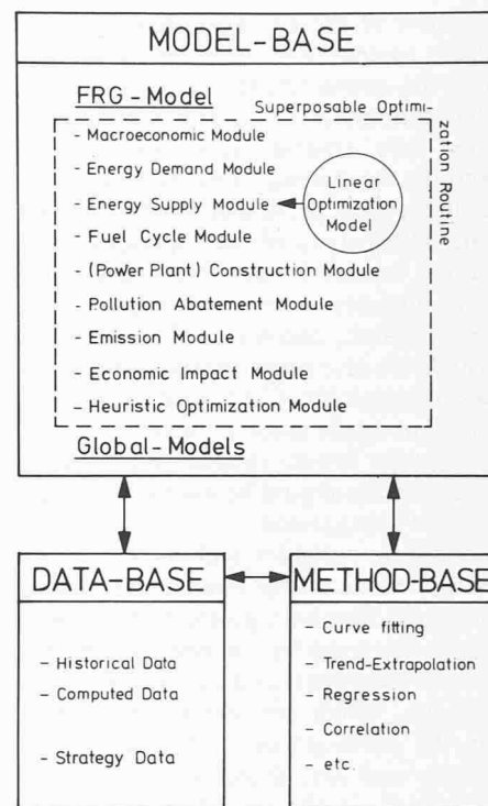
Fig. 1. The KFA-STE integrated Model System
