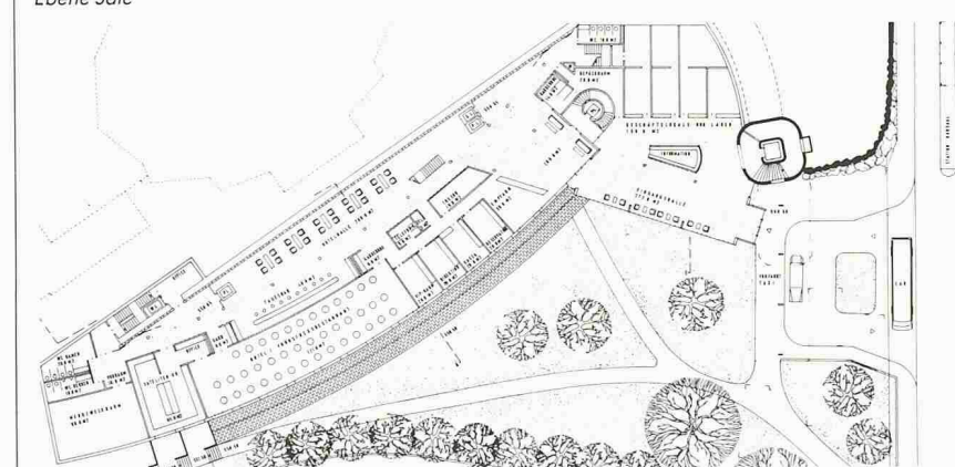
Erdgeschoss Hotel 1:1100
