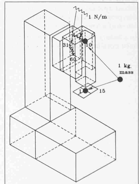
Fig. 8. Schematic view of the drilling machine
