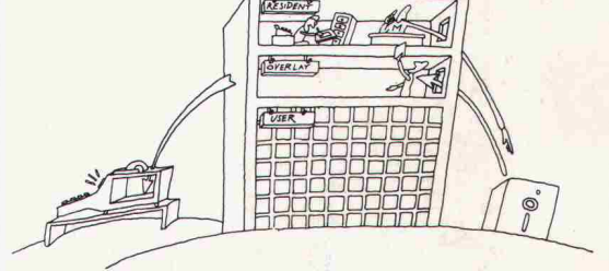
Programmsystem Büro-Administration
