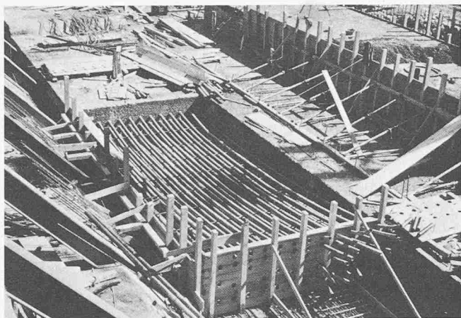
Fig. 10. Ouvrage en cours de construction Structure during building
