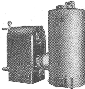
Holzgasgenerator + Patent angem.
