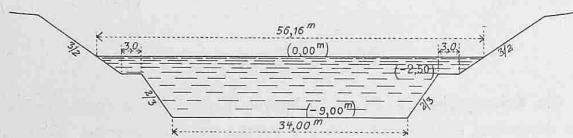
Abb. 5. Normalprofil in felsigem Terrain. — 1 : 1000.
