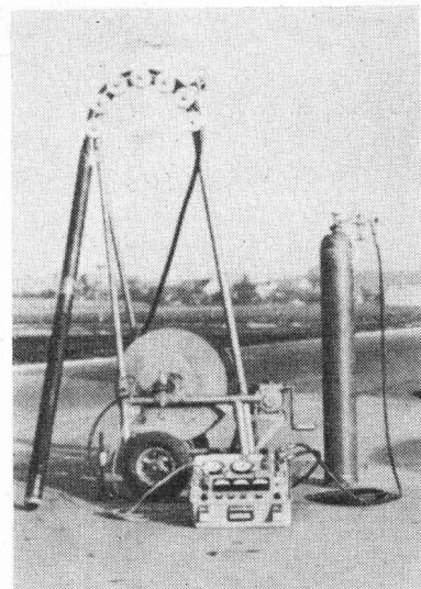
Dilatometer 95
