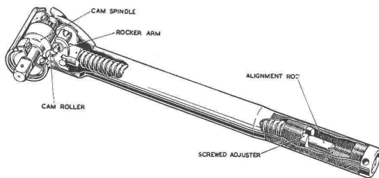
(C) "ACRATORK" TYPE TORQUE WRENCH
