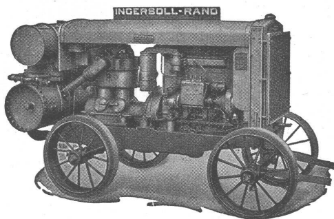
Rohölkompessor 20/26 PS.
