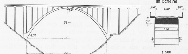
⑥ HUNDWILERTOBEL-BRÜCKE 1925
