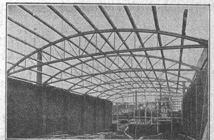
Dachbinder in Holz, System Meltzer.
