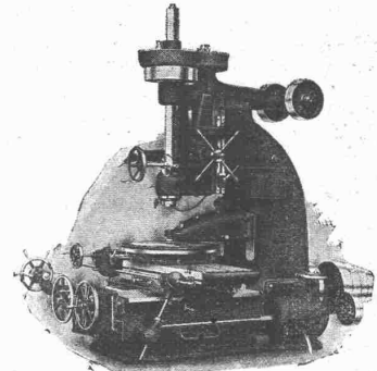
Vertikale No. 8 1575 × 865 × 660 mm.
