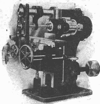
Horizontale No. 12 1060 × 300 × 525 mm.
