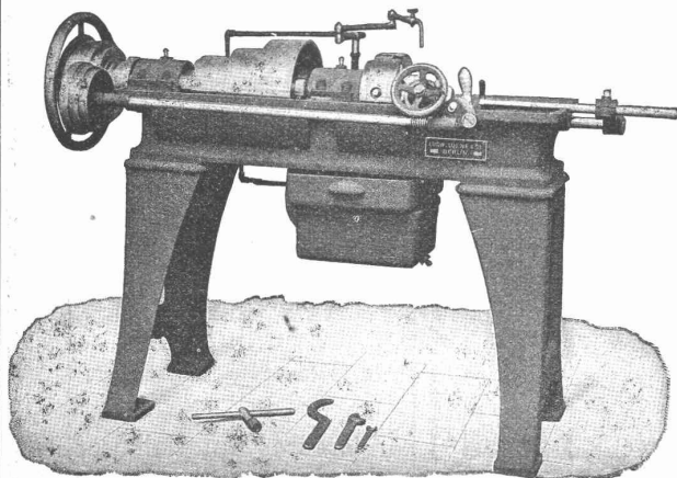
Abstechmaschine No. 7, Mod. I
