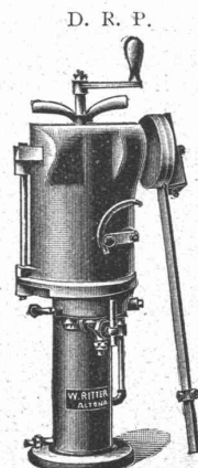
1-Stempel-Presse.
