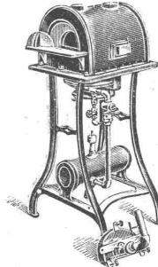
PROBIR & MUFFELOFEN
