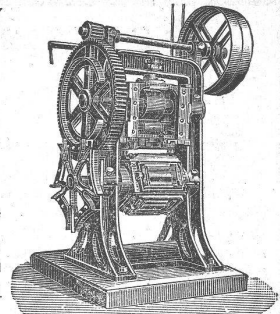
Revolver-Falzziegelpresse.
