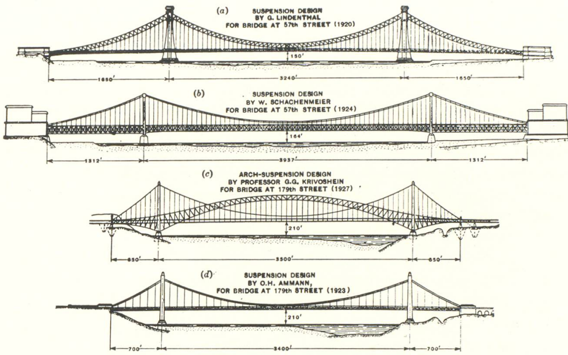
FIG. 19.—RECENT STUDIES FOR A BRIDGE ACROSS THE HUDSON RIVER.
