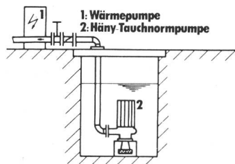
Tauchnormpumpe
