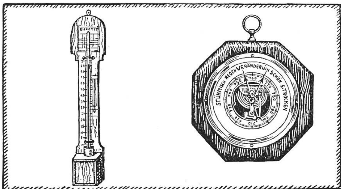
Quecksilber-Barometer.
