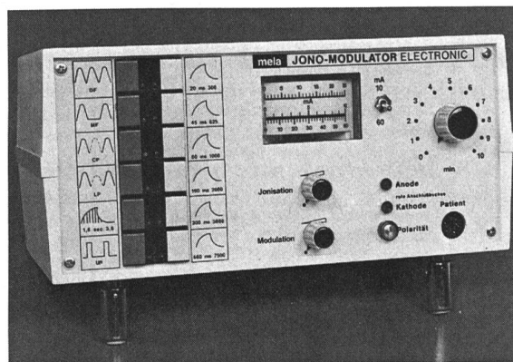
JONO-MODULATOR-ELECTRONIC
