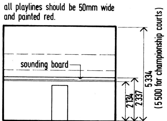
back wall
