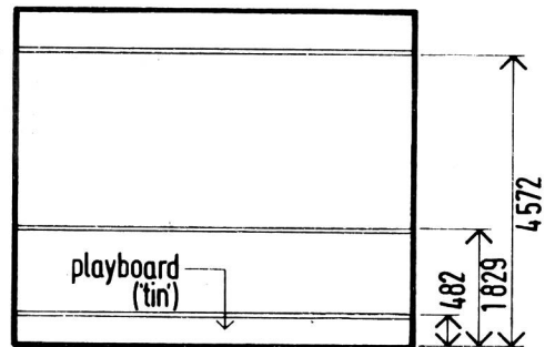
front wall
