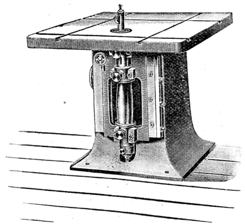
Kehlmaschine.
