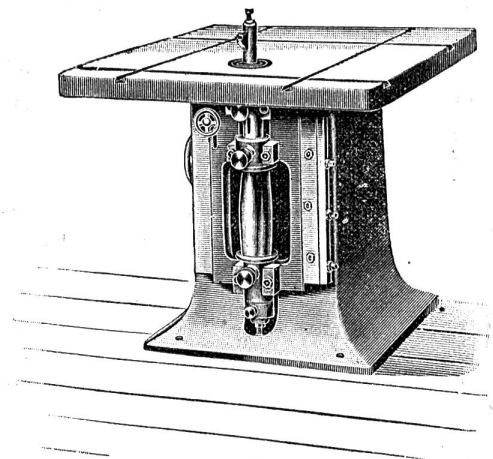
Kehlmaschine.
