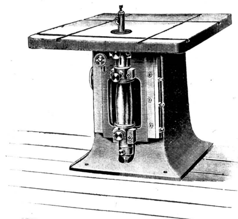
Kehlmaschine.
