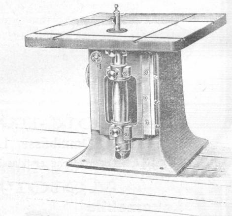
Kehlmaschine.
