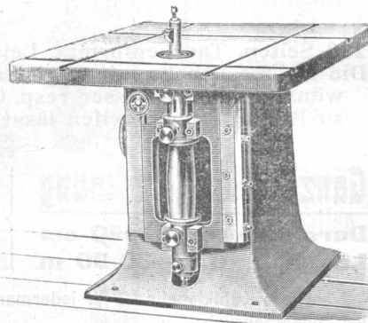
Kehlmaschine.
