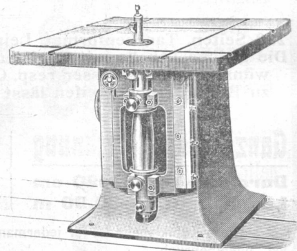
Kehlmaschine.
