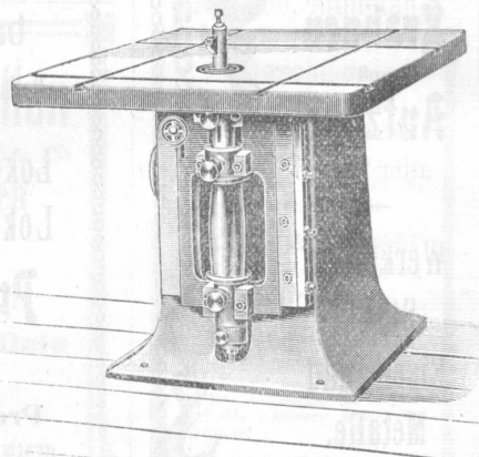
Kehlmaschine.
