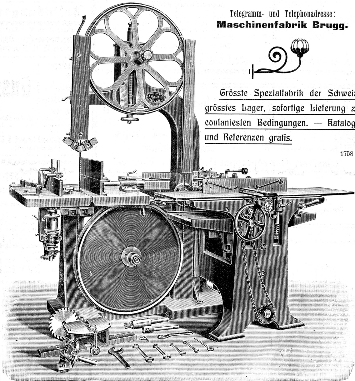
Universalmaschine No. 3.
